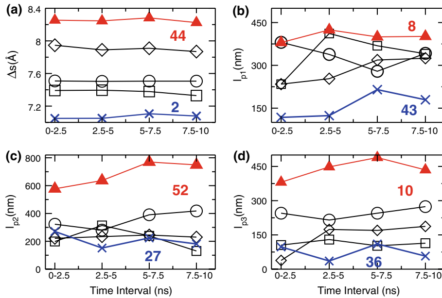
FIGURE 3. Time evolution of \Delta s and l_{pi} for select triads. Averages were made over 2.5-ns intervals, for triad 15 (circle), 30 (square), and 45 (diamond). Data for triads that occupy the minimum (blue cross) and maximum (red triangle) in Fig. 4 are also shown, with triad numbers marked.
