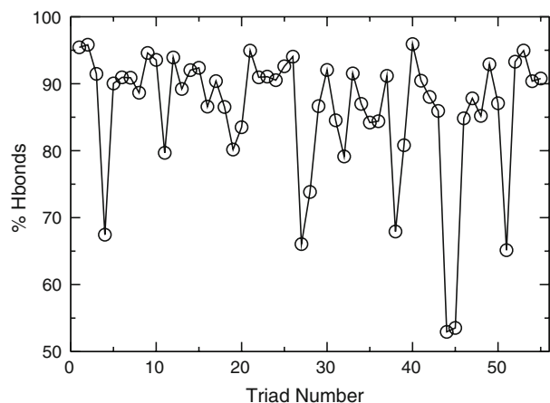
FIGURE 5. Occupancy of backbone hydrogen bonds during the simulation. A cutoff distance of 2.4 Å was used to identify hydrogen bond formation. Regions of low hydrogen bond occupancy correspond to labile regions in Fig. 4.
