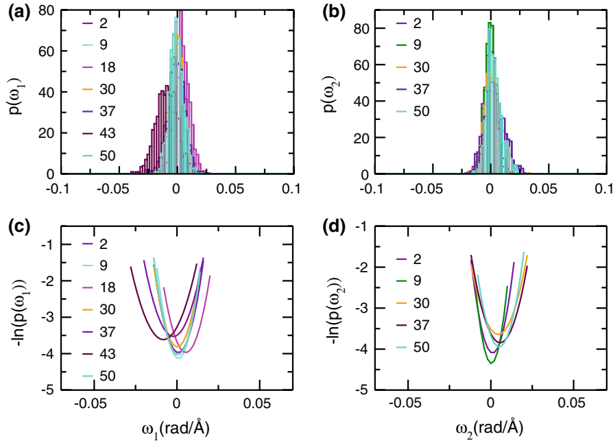
FIGURE 2. Example distributions of (a) \omega_1 and (b) \omega_2 , and (c, d) quadratic fits to their logarithm. Corresponding triad numbers are marked in the graph. While equilibrium curvatures \omega_{01} & \omega_{02} are generally 0 along the length of tropomyosin, at triad 43 (lowest rigidity region Fig. 4b) \omega_{01} is about -0.01 .
