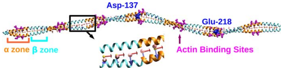
FIGURE 1. Crystal structure of a cardiac muscle tropomyosin (PDB ID:1C1G). 32 The \alpha and \beta zones are shown in orange and cyan, respectively. Successive \alpha or \beta zones rotate by about 90^\circ axially. Side chains of the putative actin binding residues 17 in \alpha zones are shown in magenta. Asp137 and Glu218 are shown in blue van der Waals representation. Starting with triad 1 on the left (N-terminus), we assigned 56 triads along the length of the molecule in intervals of five residues. Triads 1 and 56 were not considered for the flexibility map to eliminate edge effects. The magnified image shows triads 14–18. \mathbf{e}_3 (red) points to the right, \mathbf{e}_2 (blue) points downward, and \mathbf{e}_1 (pink) points out of the page.
