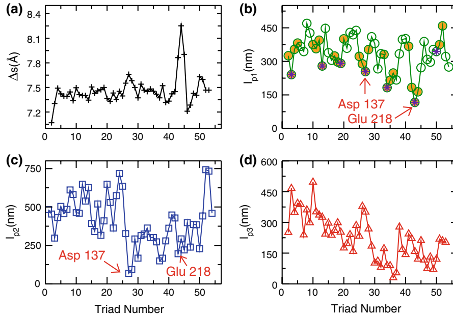
FIGURE 4. Flexibility map of tropomyosin. (a) \Delta s , showing a jump near the most labile region at Glu218 (triad 43). (b) l_{p1} regarding local splay deformation. Minimum occurs again at triad 43. Marked in orange represent \alpha zones (cf., Fig. 1), which contain actin binding sites (magenta stars) that are locally the most flexible. (c) l_{p2} regarding bend of the broad face. (d) l_{p3} representing torsional stiffness. Overall, the molecule is more flexible toward the C-terminus.
